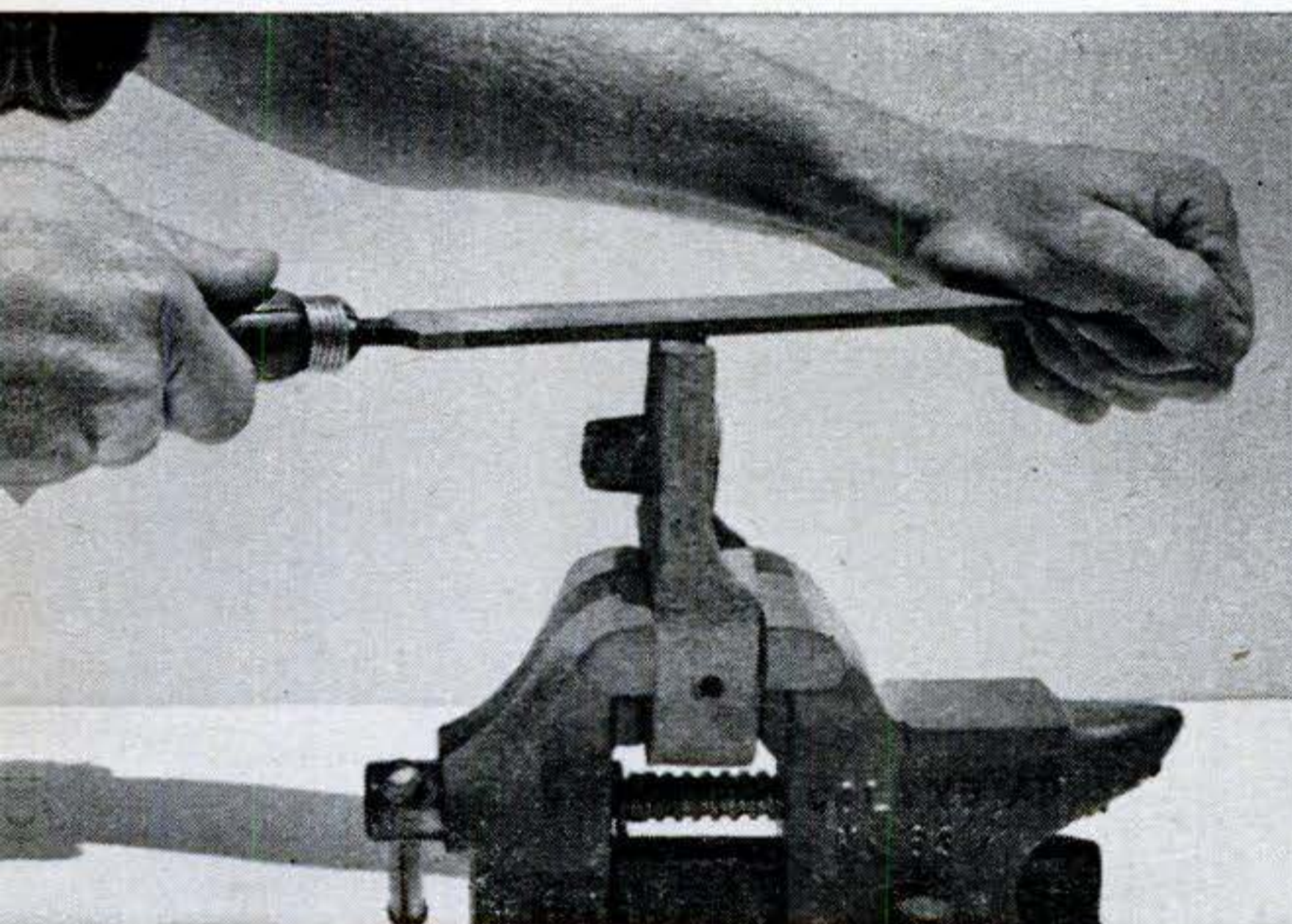
HERE'S A GOOD GRIP for heavy filing. Have work at elbow height and stand erect to avoid rocking-horse strokes.
